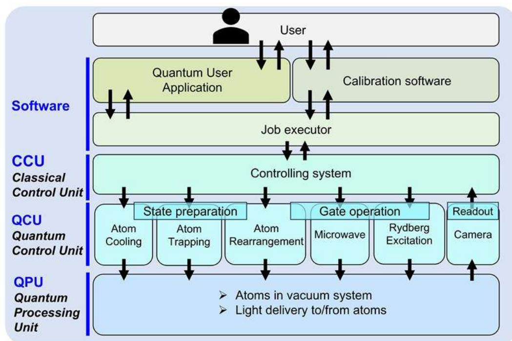
Fig.2 Layer structure of the full-stack neutral-atom quantum computer "Shunkai".
