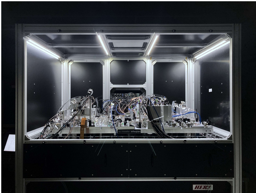
Fig.1 Japan's first neutral-atom full-stack quantum computer “春海-Shunkai”. (Photography by Takafumi Tomita)
